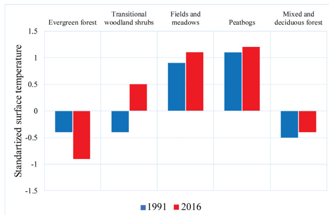
Fig. 2. Modus values of relative surface temperature for land cover categories.
