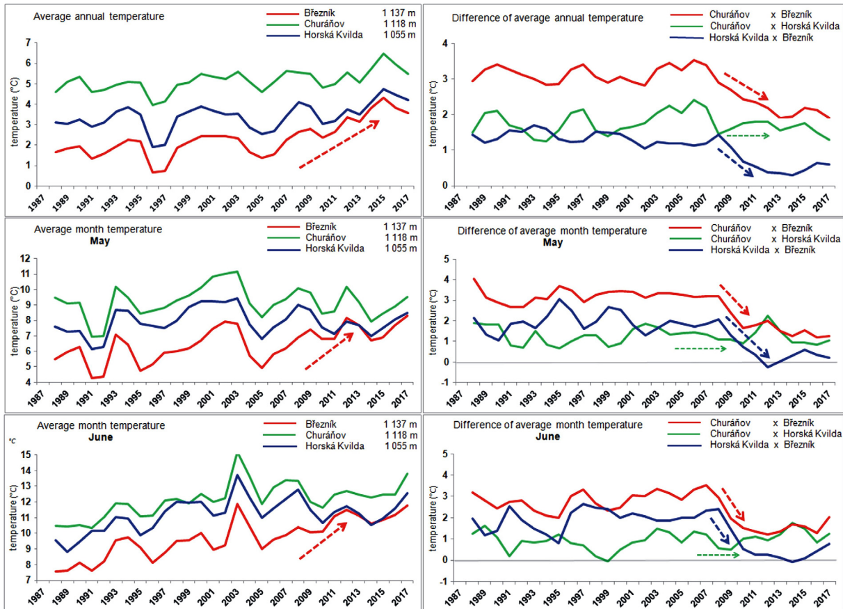
Fig. 7. Average annual temperature at the meteorological stations of Březník (1137 m a.s.l.), Churáňov (1118 m a.s.l.) and Horská Kvilda (1055 m a.s.l.). Air temperature differences (in °C) between Churáňov station x Březník and Churáňov x Horská Kvilda between 1988 and 2017 (Data source: CHMI and A. Vojvodík – operator of amateur meteorological stations).
